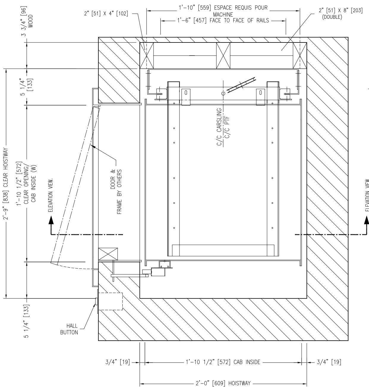
PLAN VIEW
