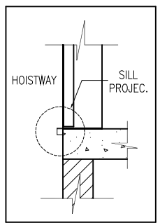
SILL DETAIL
