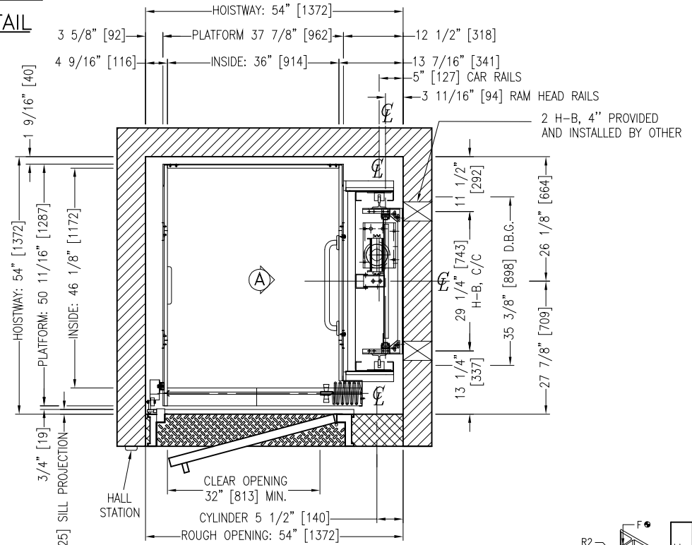
PLAN OF HATCH
