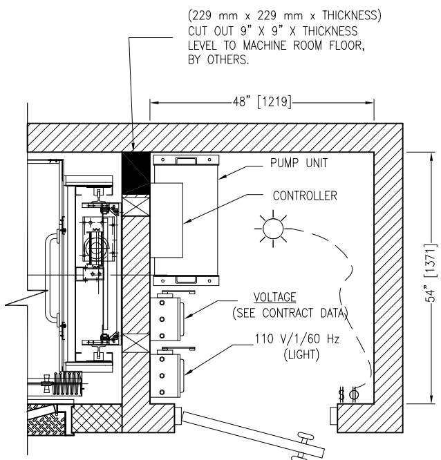
TYPICAL MACHINE ROOM PLAN
