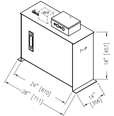
POWER UNIT
