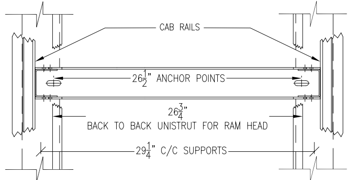
RAIL BRACKET DETAIL
