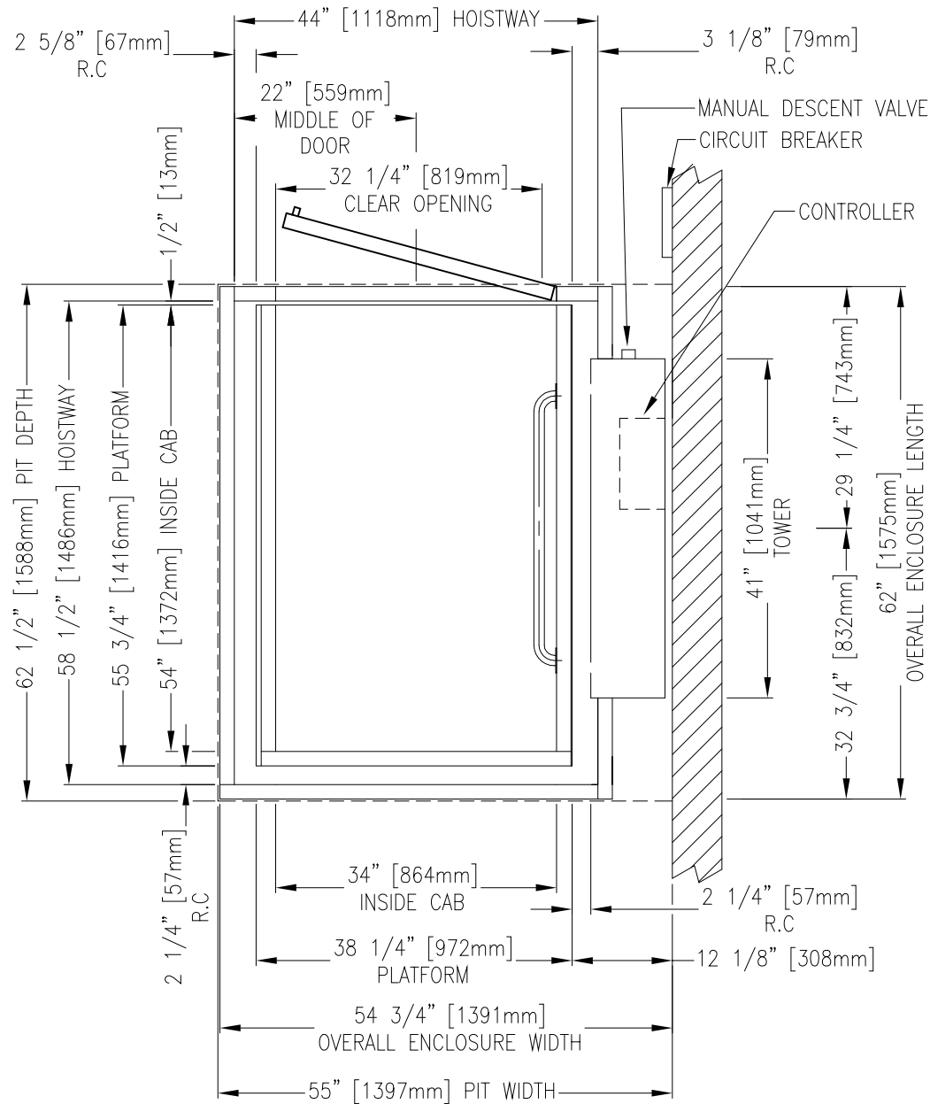
HOISTWAY LAYOUT
