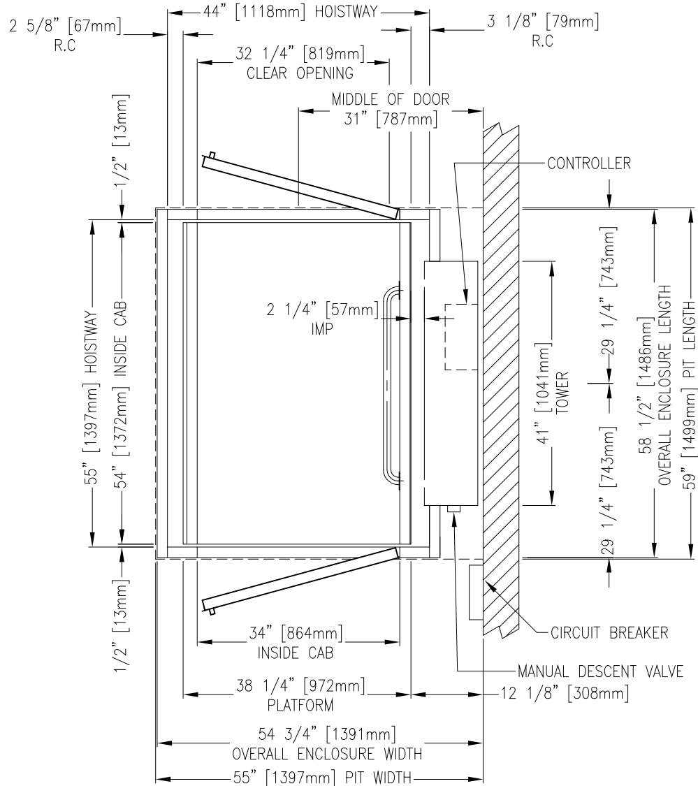
HOISTWAY LAYOUT
