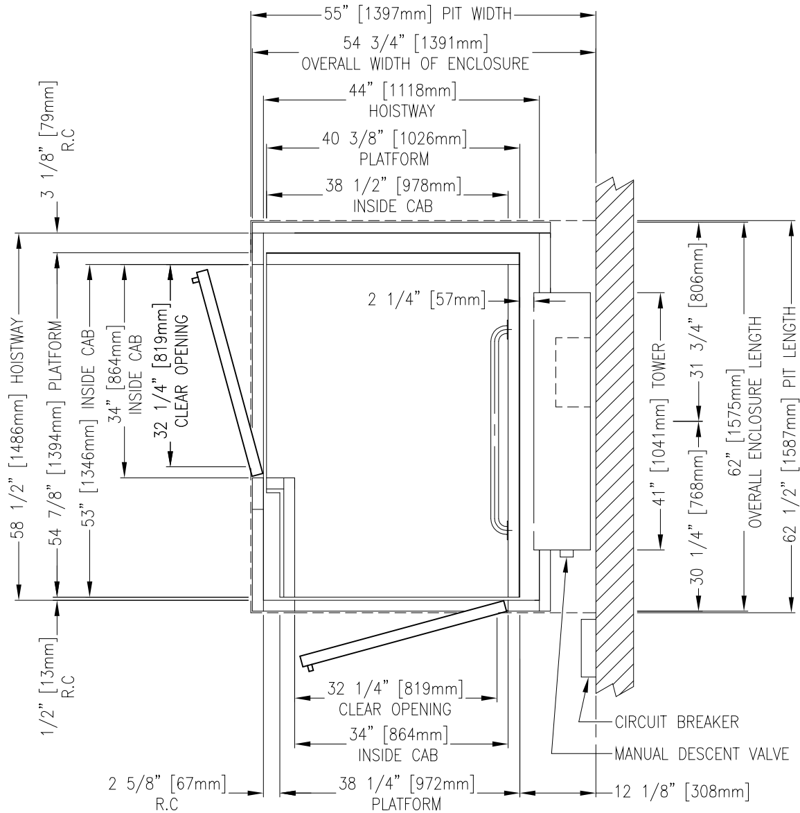
HOISTWAY LAYOUT
