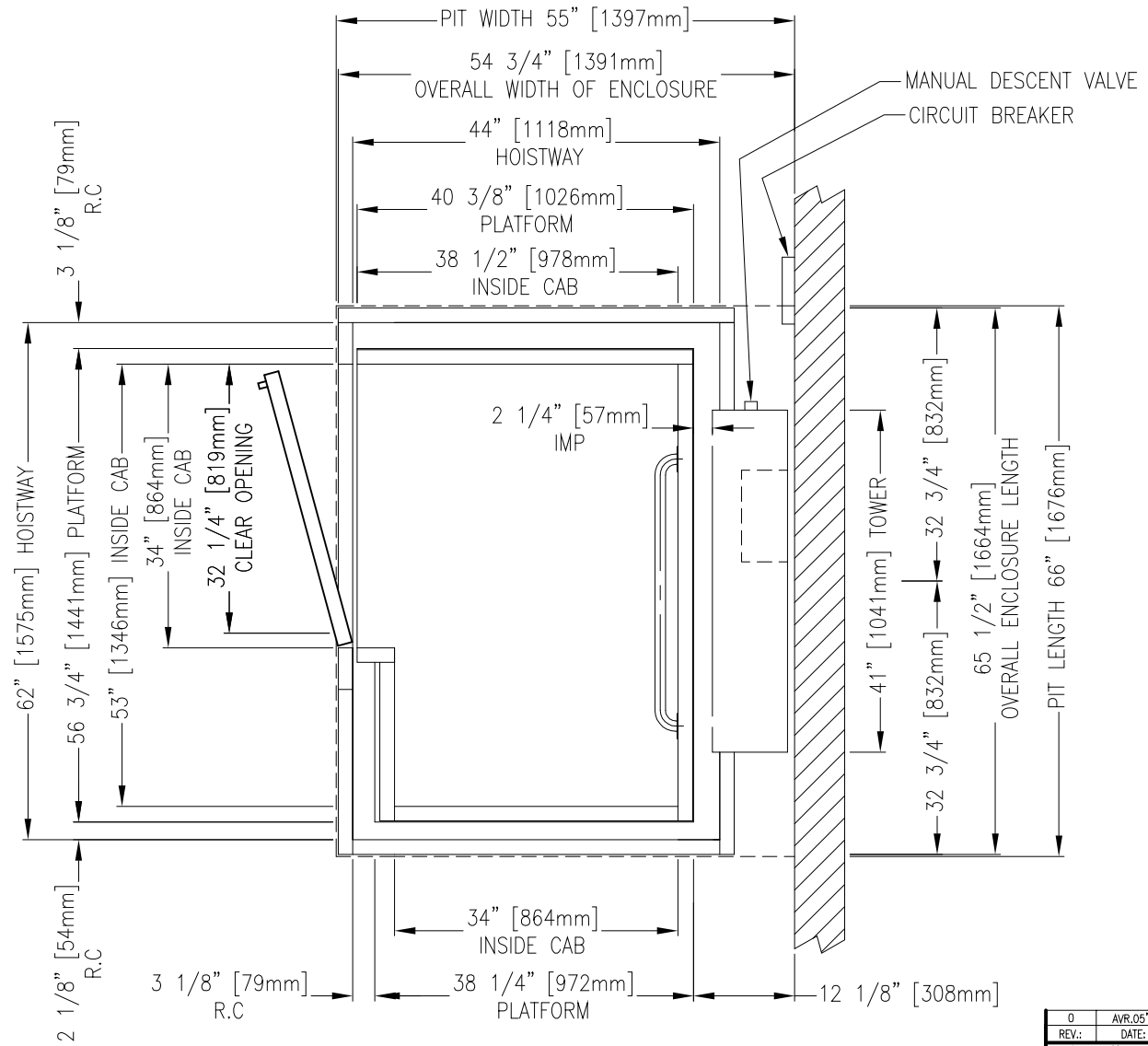
HOISTWAY LAYOUT
