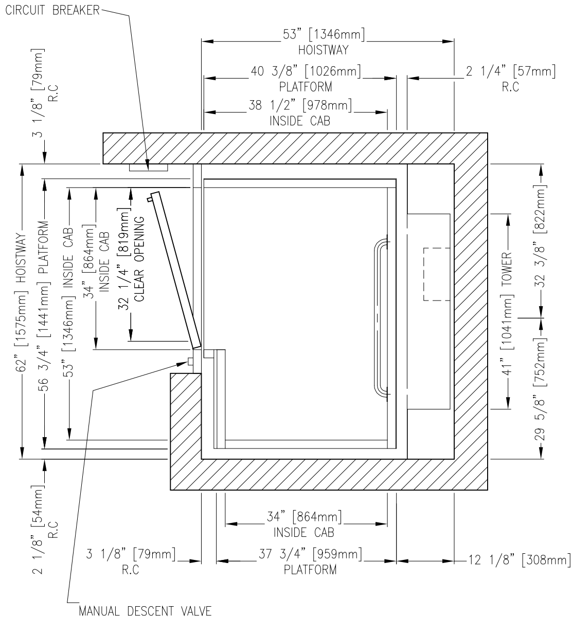
HOISTWAY LAYOUT
